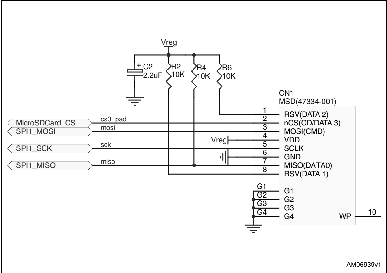
Figure 5. MicroSD
