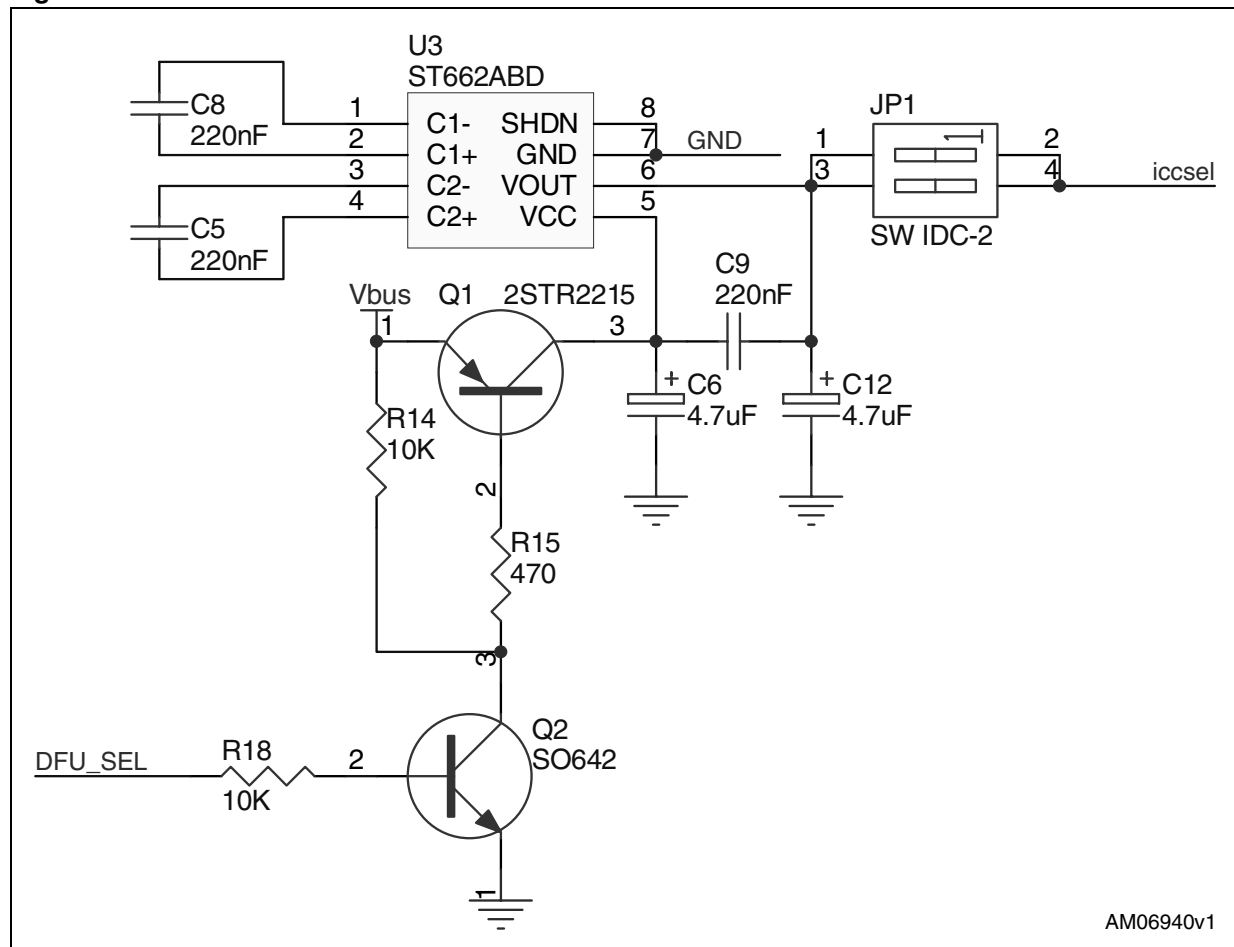
Figure 6. DFU
