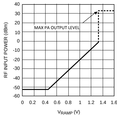
Figure 26. P IN vs. V RAMP
