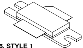
CASE 465-06, STYLE 1 NI-780 MRF18085ALR3
