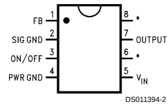
8-Lead DIP
