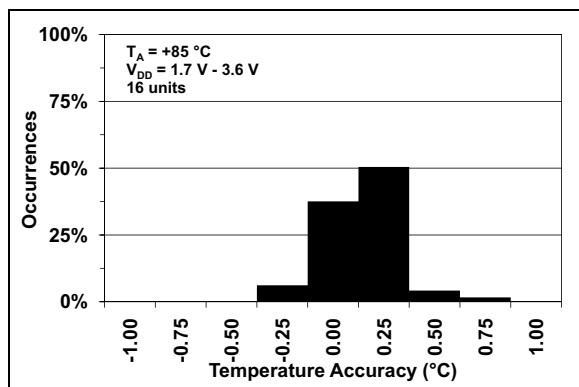
FIGURE 2-2: Temperature Accuracy Histogram, T_A = +85^\circ\text{C} .
