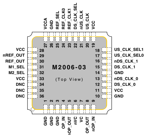
Figure 1: Pin Assignment
