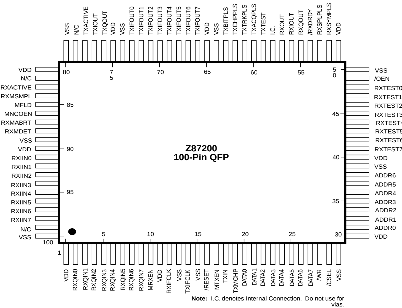
Figure 2. Z87200 100-Pin PQFP Pin Description
