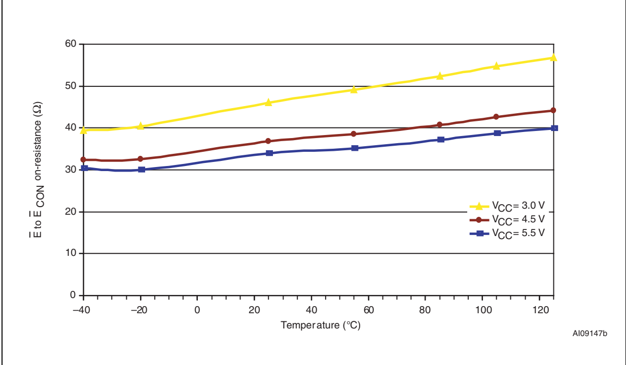
Figure 24. \bar{E} to \bar{E}_{CON} on-resistance vs. temperature
