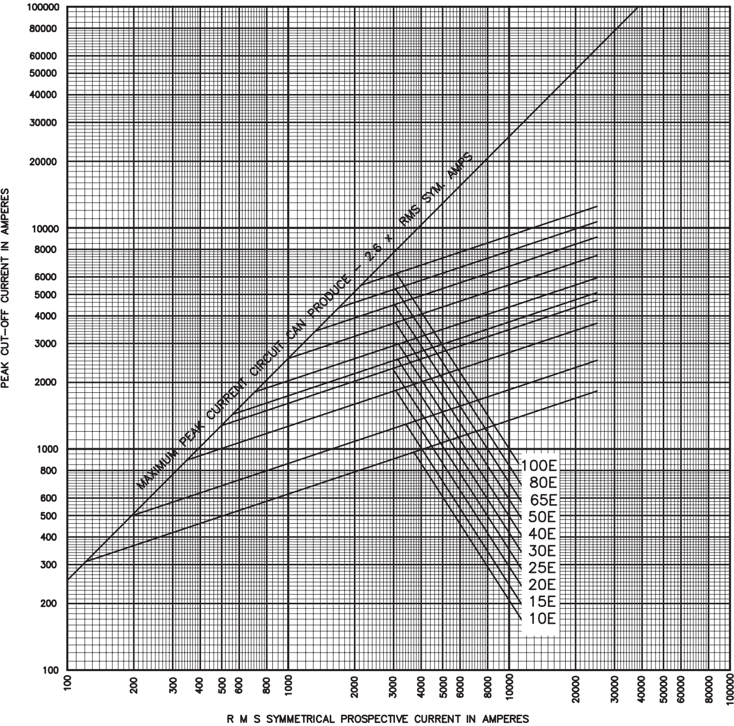
25.8 to 38 kV cut-off curves
