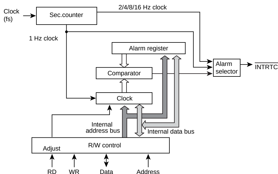
Figure 26-1 Block Diagram
