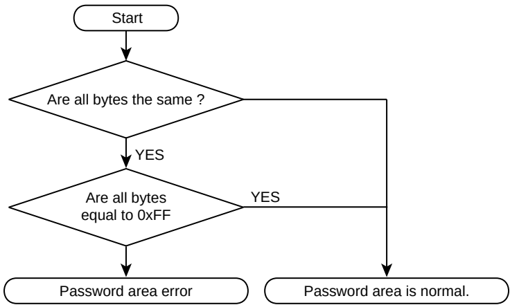
Figure 31-7 Password Area Verification Flowchart (1)
