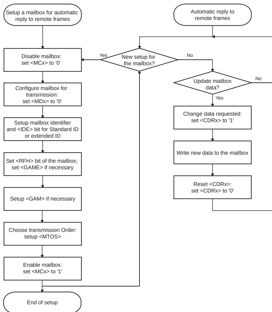
Figure 20-11 Flowchart of Remote Frame Handling Using the Automatic Reply Feature
