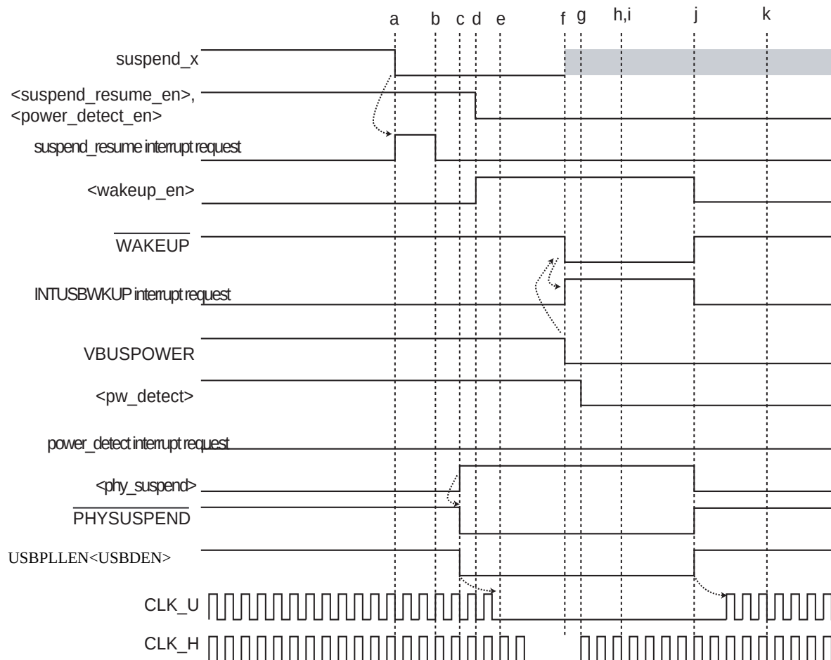
Figure 18-19 Operation of suspend/disconnect signals (to stop CLK_H)
