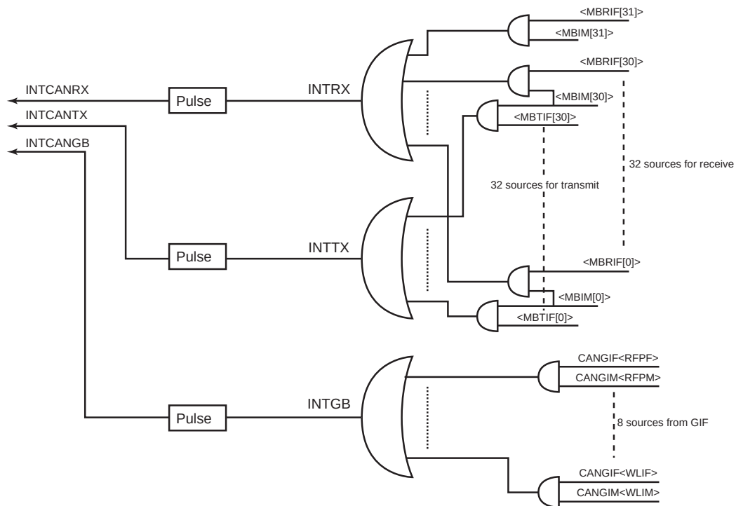
Figure 20-6 Block Diagram of CAN interrupt signals
