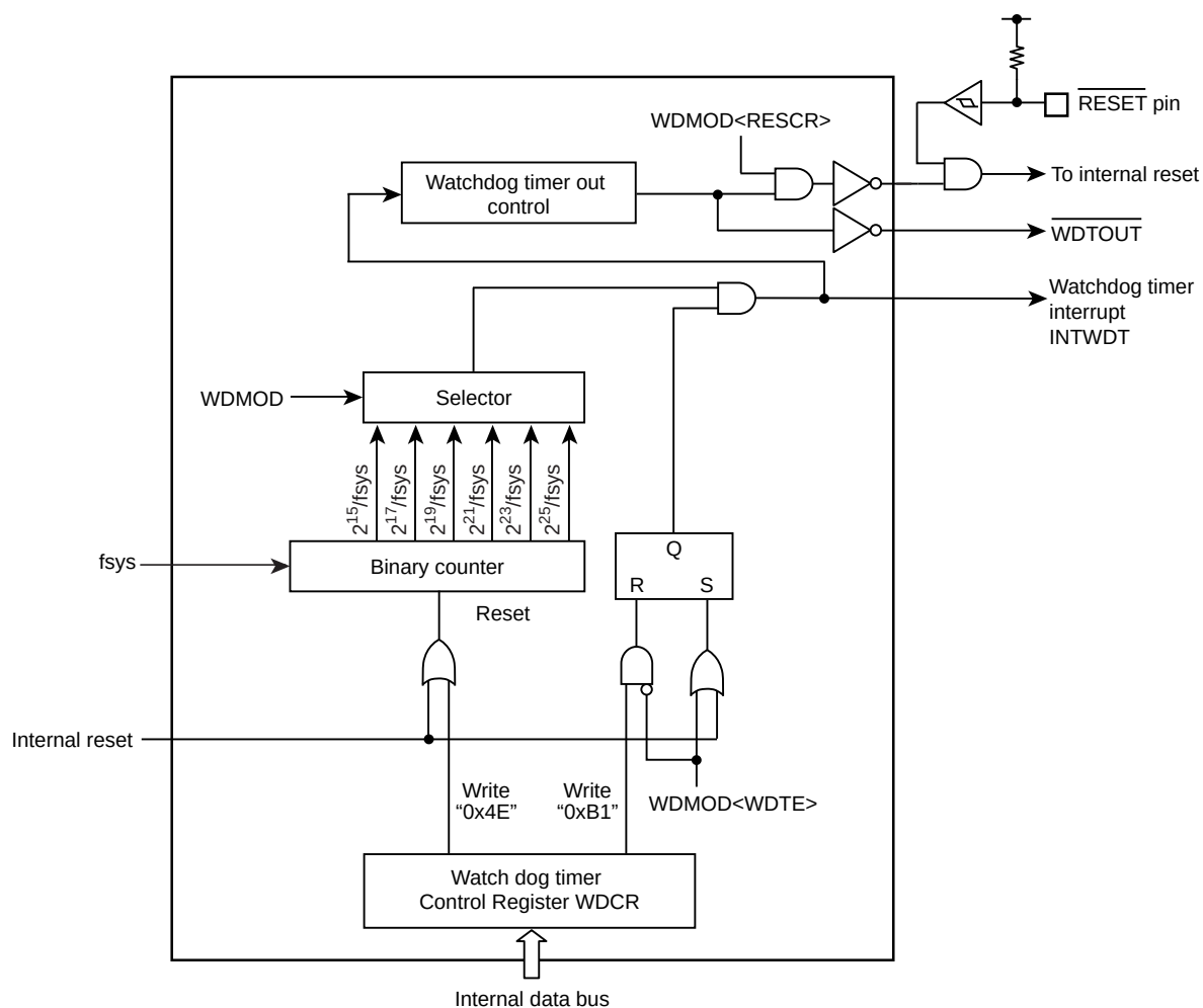
Figure 30-1 Block Diagram of the Watchdog Timer
