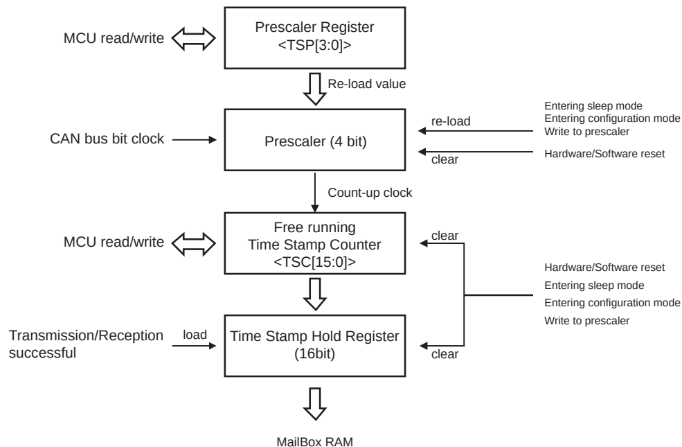
Figure 20-5 Timer Stamp Counter
