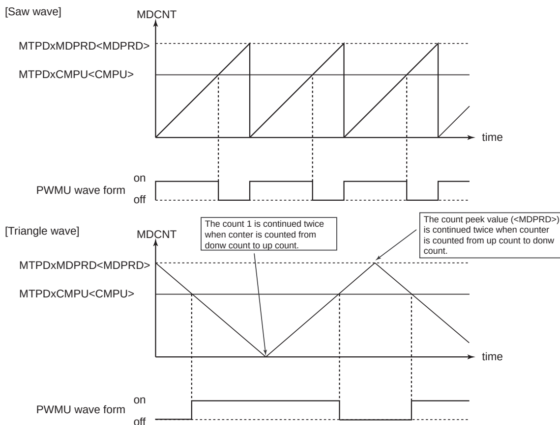
Figure 24-23 PWM waveform
