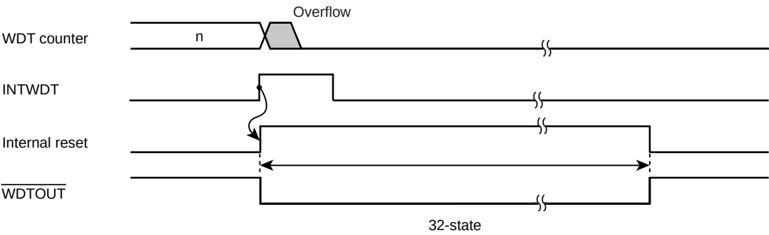
Figure 30-3 Internal reset generation
