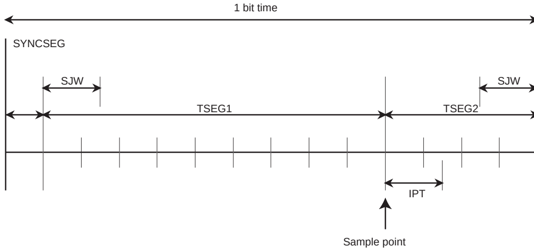
Figure 20-12 CAN Bit Timing
