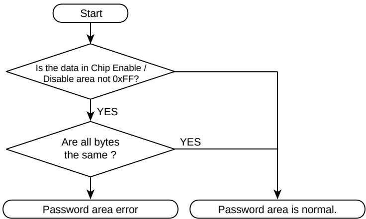
Figure 31-8 Password Area Verification Flowchart (2)
