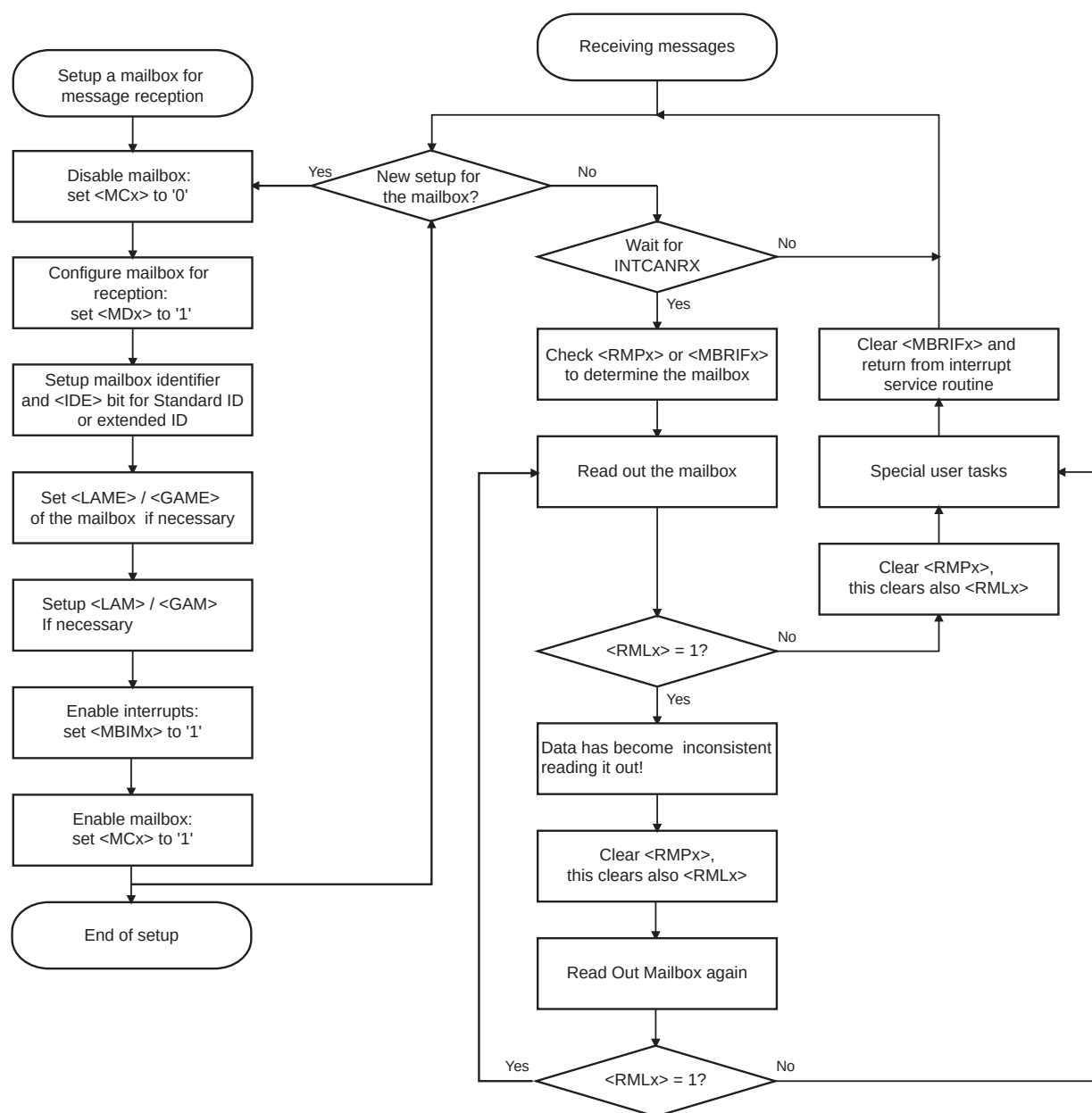
Figure 20-9 Flowchart of Message Reception
