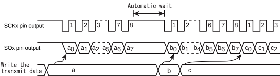
Figure 15-15 Automatic Wait
