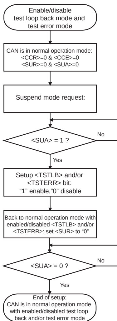
Figure 20-8 Flowchart of Setup of Test Loop Back Mode and Test Error Mode
