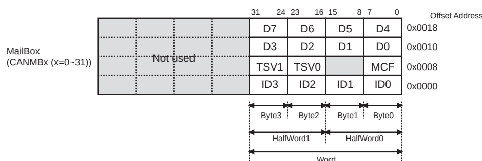
Figure 20-2 Configuration of Mailboxes
