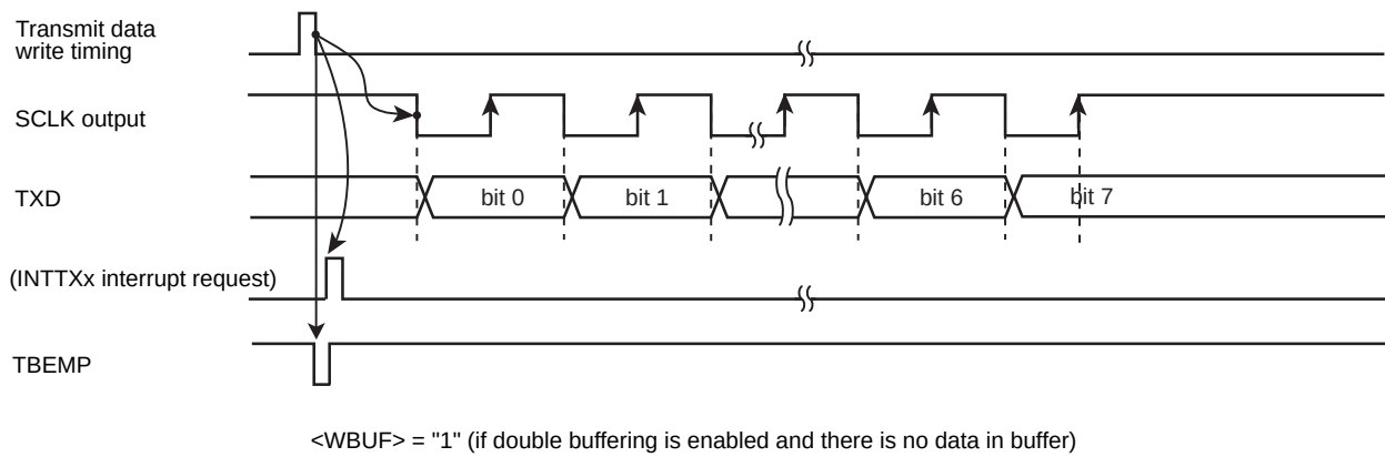
Figure 13-12 Transmit Operation in the I/O Interface Mode (SCLK Output Mode)
