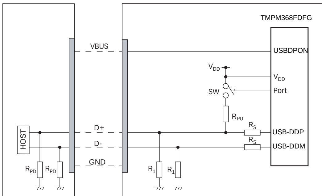
Figure 18-6 Connection example of the USB bus and TMPM368FDFG.
