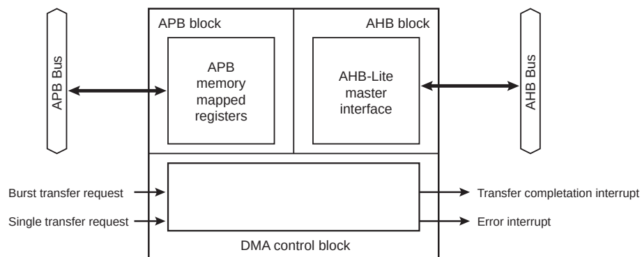
Figure 9-1 Micro DMA Block Diagram (common to the Unit A and B)
