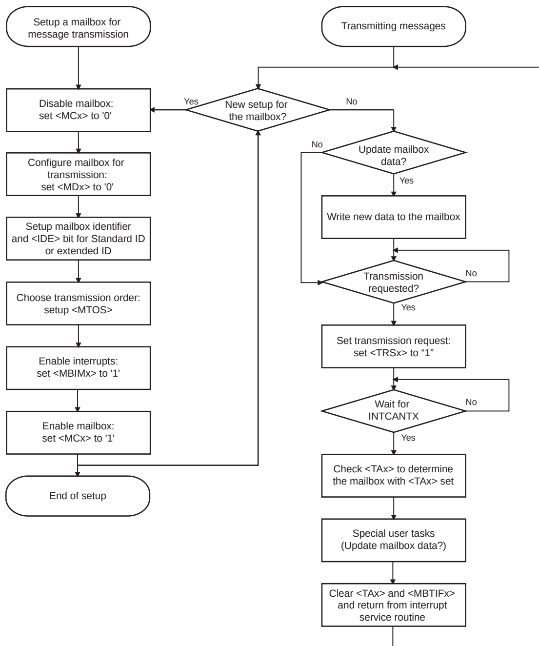
Figure 20-10 Flowchart of Message Transmission
