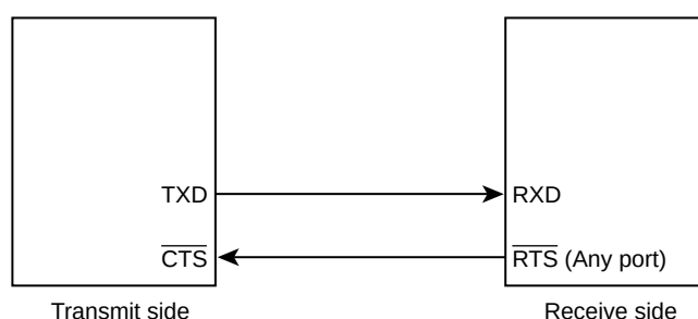
Figure 13-8 Handshake Function
