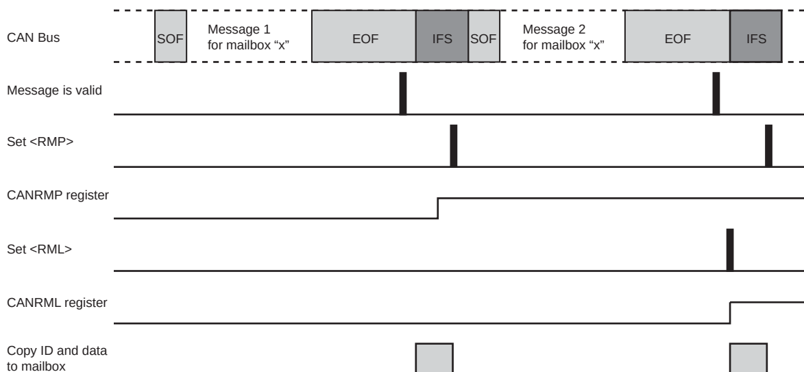
Figure 20-3 Timing when a Receive Message Lost Occurs
