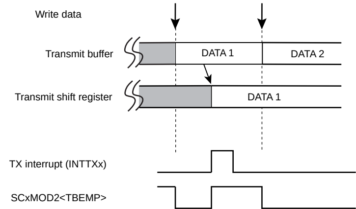
Figure 13-7 Operation of Transmission Buffer (Double buffer is enabled)
