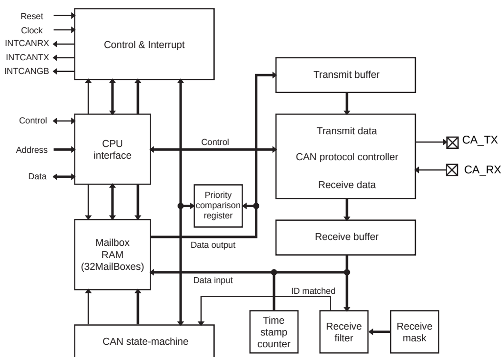
Figure 20-1 Block Diagram of CAN controller
