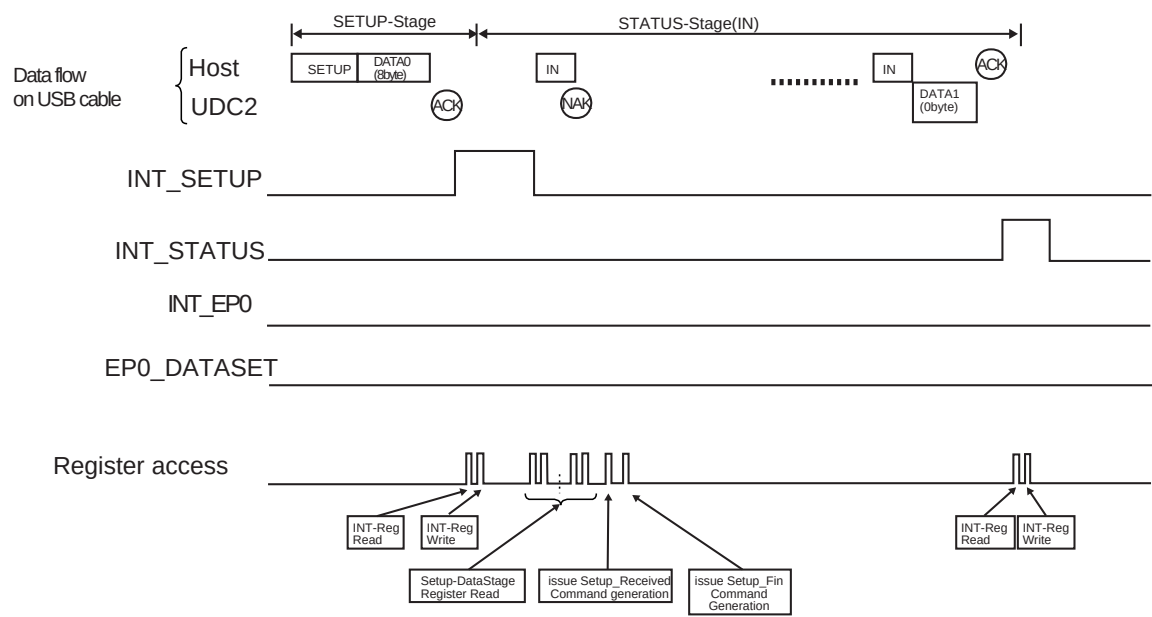
Figure 18-23 Flow of control in Control-WR transfer (without DATA-Stage)
