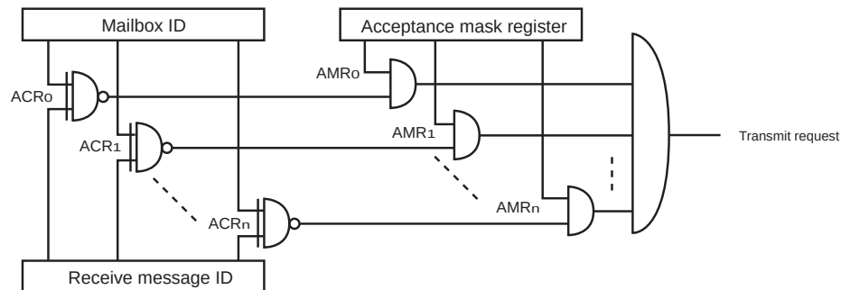
Figure 20-4 Receive filtering
