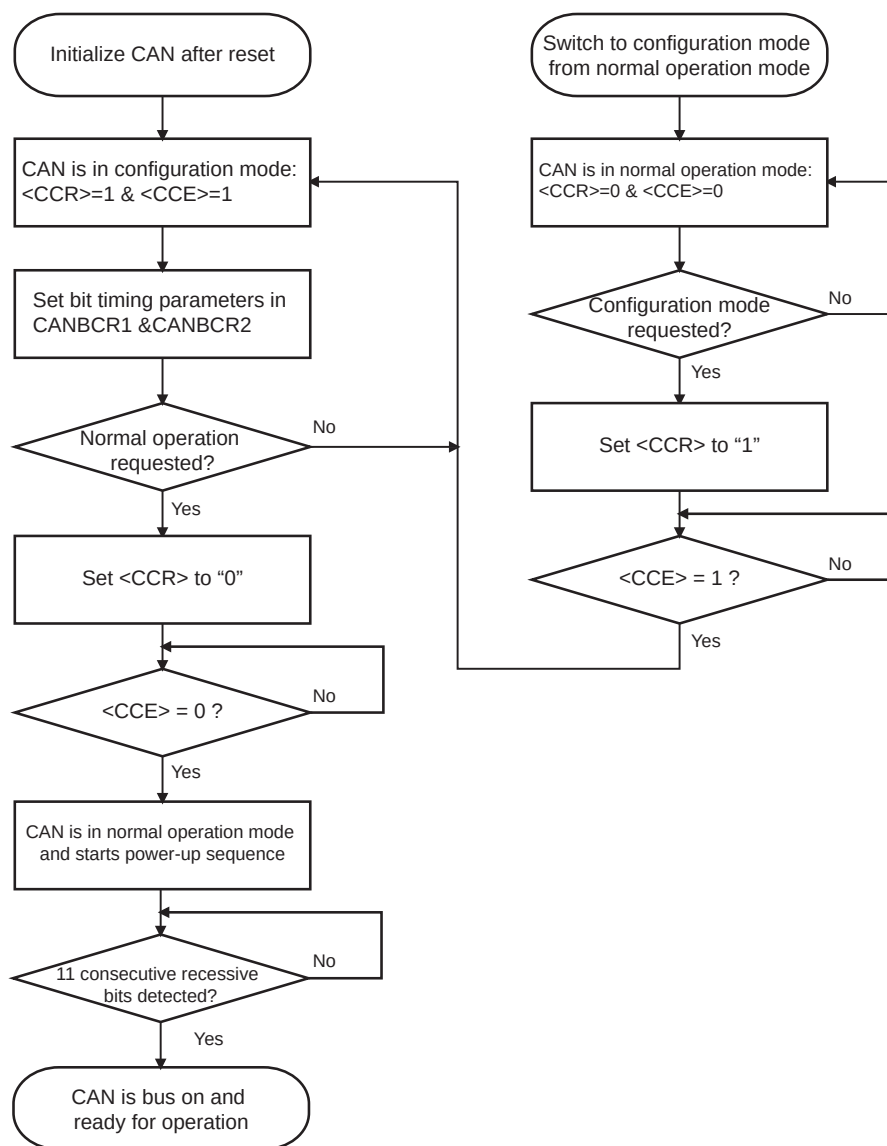
Figure 20-7 Flowchart of Initial Setup of CAN Controller
