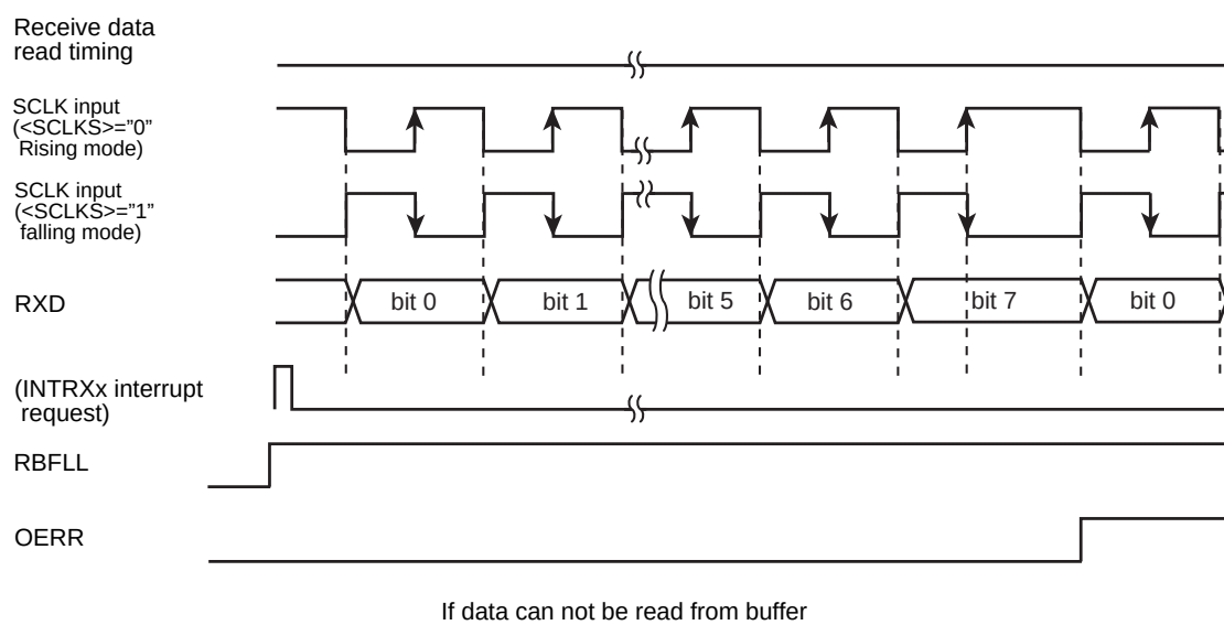
Figure 13-15 Receive Operation in the I/O Interface Mode (SCLK Input Mode)
