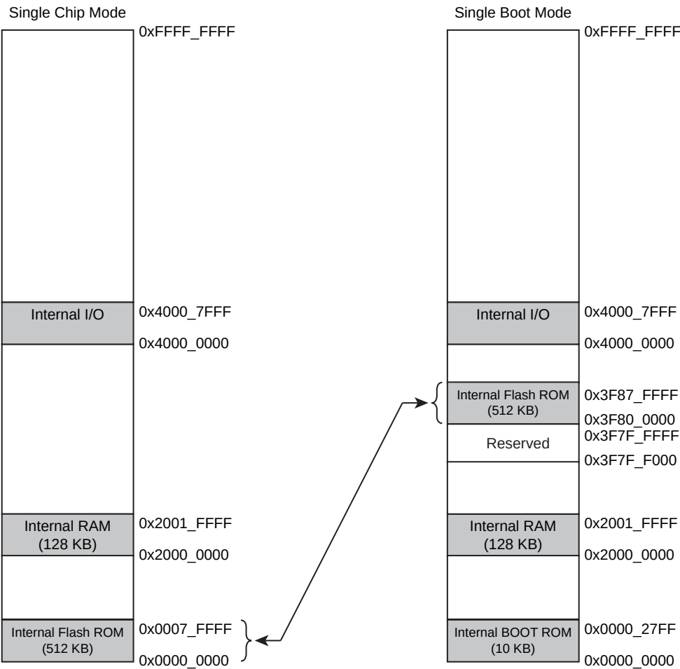
Figure 31-3 Memory Maps for TMPM368FDFG
