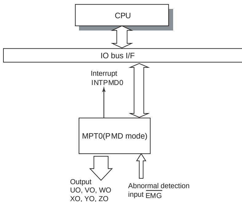
Figure 24-20 Block diagram of related with motor control
