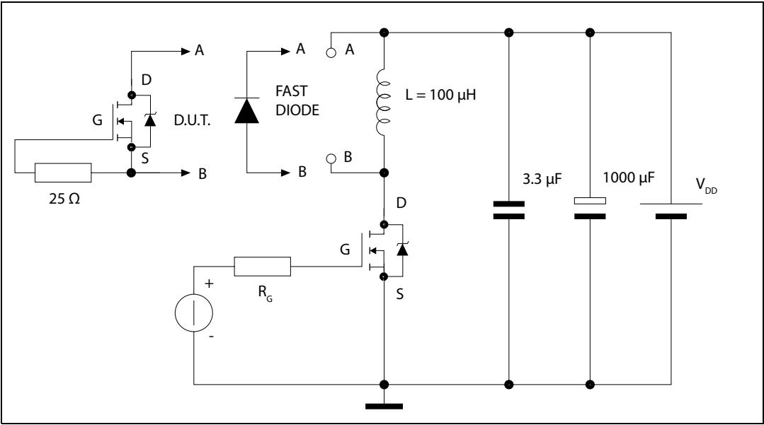
Figure 5. Test circuit for inductive load switching and diode recovery times
