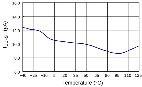
Figure 8. Startup Current
