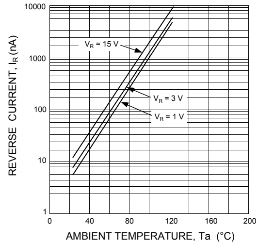
FIG. 6 - REVERSE CURRENT VS. AMBIENT TEMPERATURE : MA700
