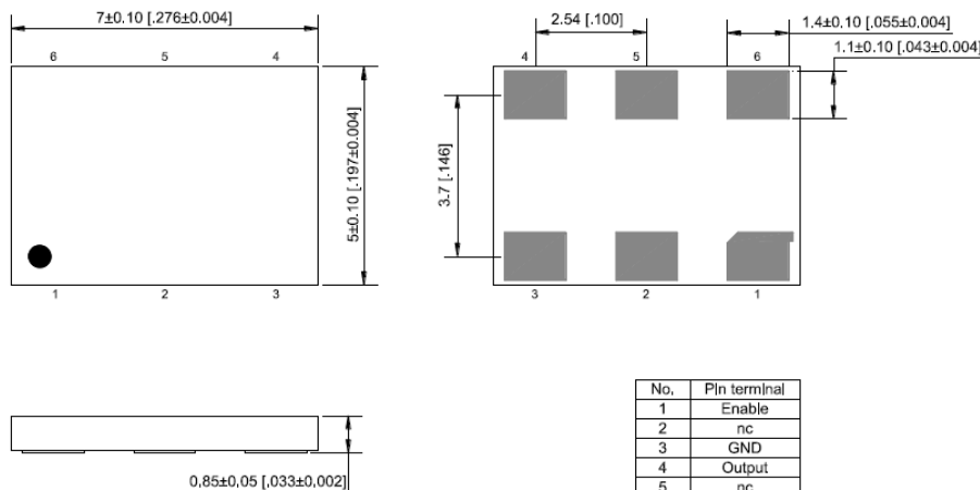
External Dimensions
