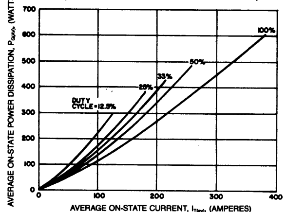
MAXIMUM ON-STATE POWER DISSIPATION (RECTANGULAR WAVEFORM — EXTENDED)
