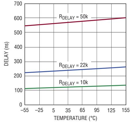
PG Rising Delay Time vs Temperature
