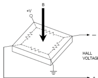
Dwg. AH-011-2
