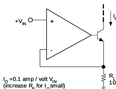
High Compliance Current Sink
