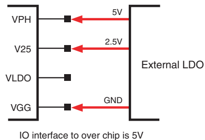
Case A. VPH: External 5V VLDO: External 2.5V (Internal LDO Off: Register Control)
