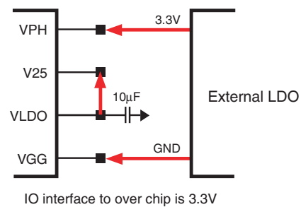
Case D. VPH: External 3.3V VLDO: Internal LDO 2.5V
