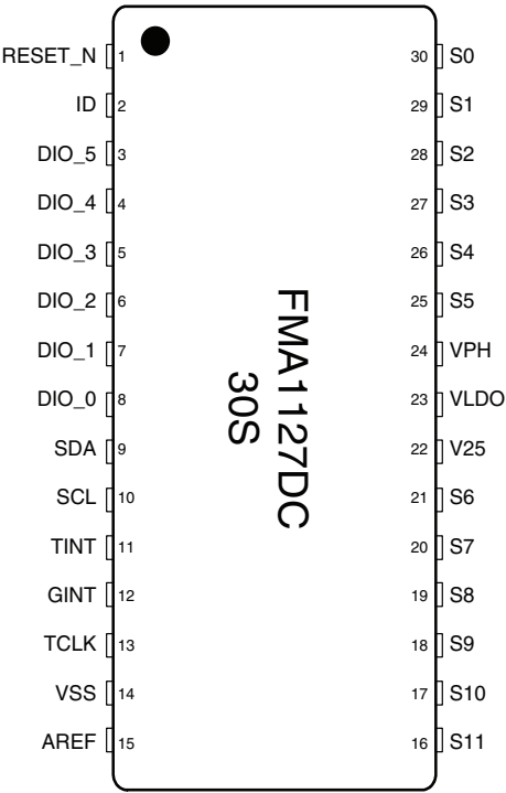
30-Pin SSOP
