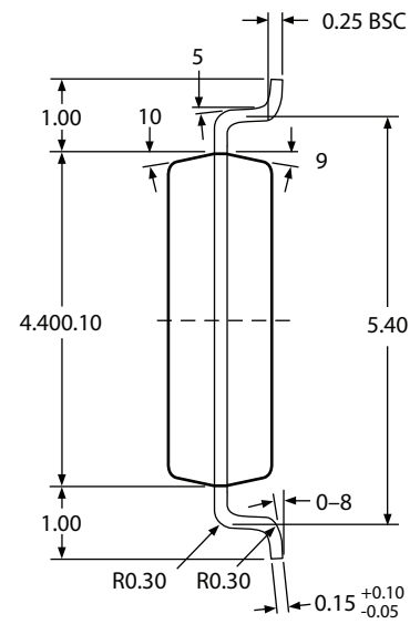
End View
