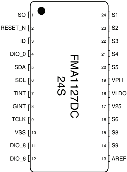
24-Pin SSOP
