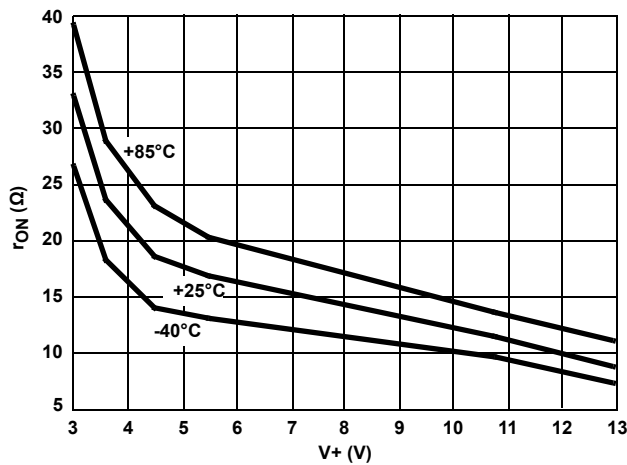
FIGURE 9. ON-RESISTANCE vs SUPPLY VOLTAGE
