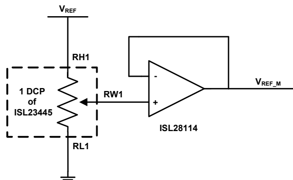
FIGURE 2. V_{\text{REF}} ADJUSTMENT
