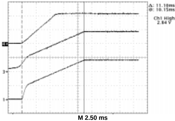
Figure 4. CS5156 Demonstration Board Startup in Response to Increasing 12 V and 5.0 V Input Voltages. Extended Off Time is Followed by Normal Off Time Operation when Output Voltage Achieves Regulation to the Error Amplifier Output.
