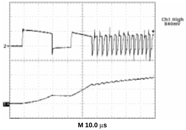
Figure 6. CS5156 Demonstration Board Enable Startup Waveforms
