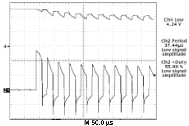
Figure 12. CS5156 Demonstration Board Hiccup Mode Short Circuit Protection. Gate Pulses are Delivered While the Soft Start Capacitor Charges, and Cease During Discharge
