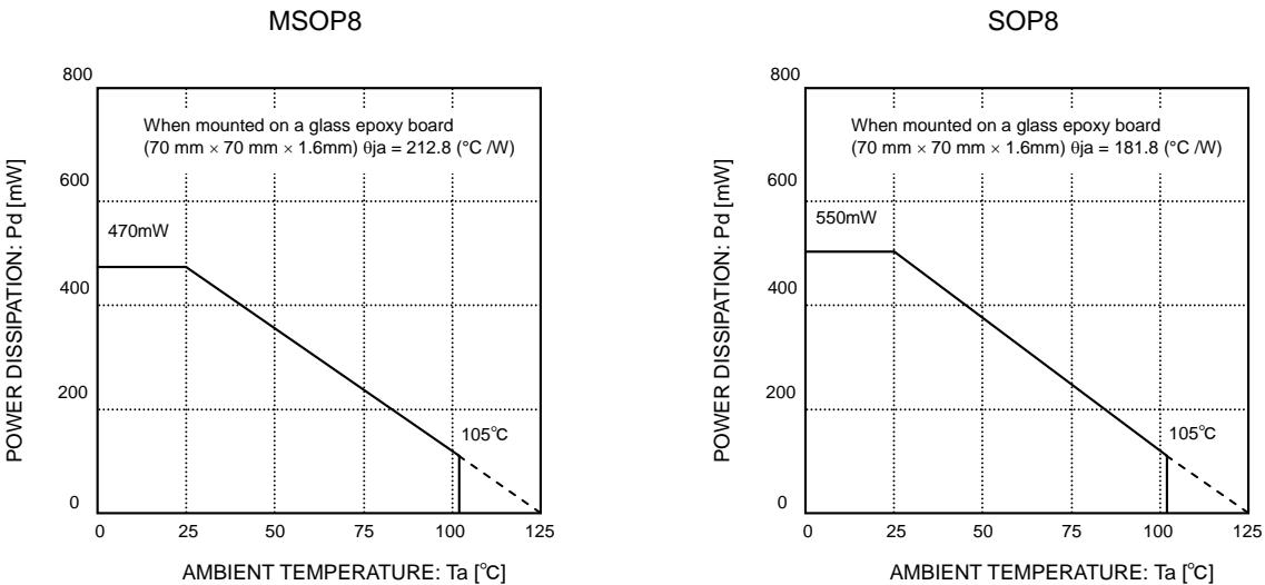
Figure 16. Power Dissipation
