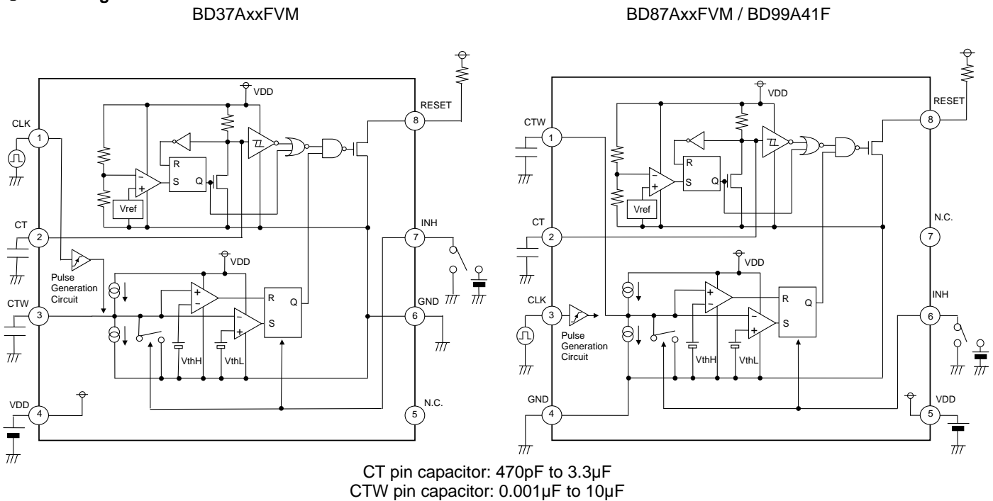
Figure 2. Block Diagrams
