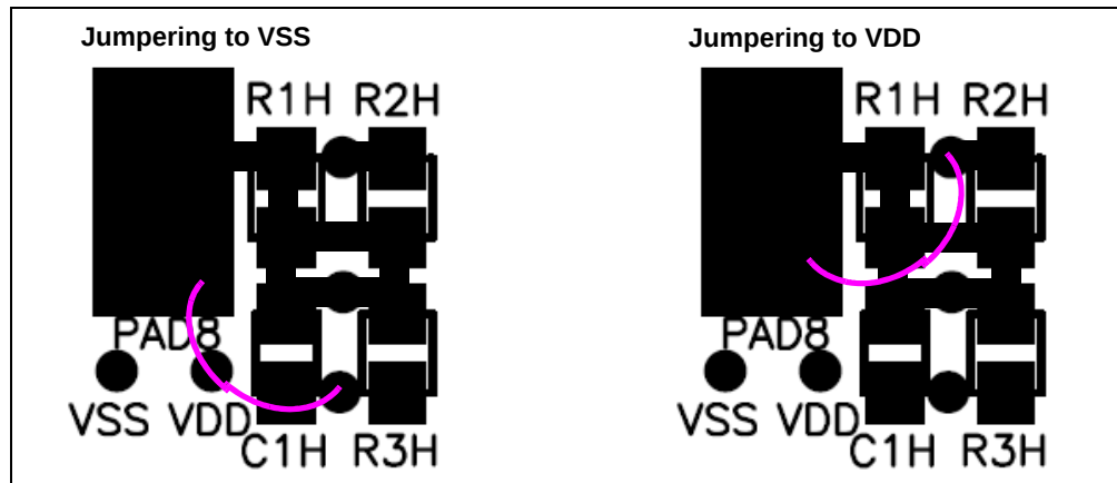
FIGURE D-3: Alternate Jumping the PCB pad to either V_{SS} or V_{DD} .
