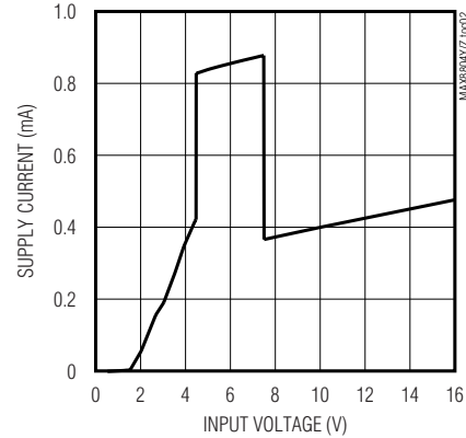
SUPPLY CURRENT vs. INPUT VOLTAGE (USB CHARGING MODE)
