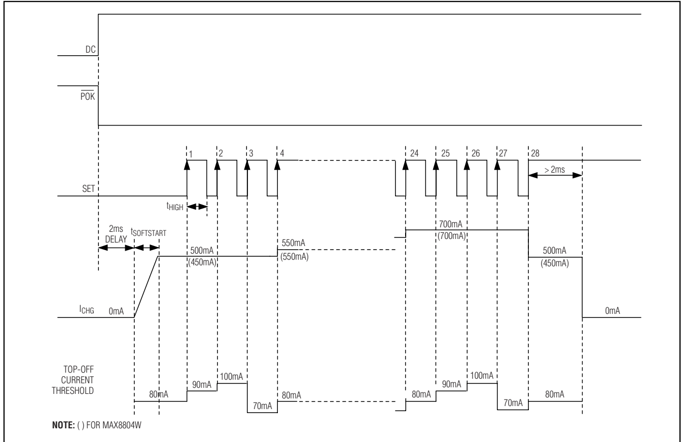
Figure 3. DC Charging Current and Top-Off Threshold Programming
