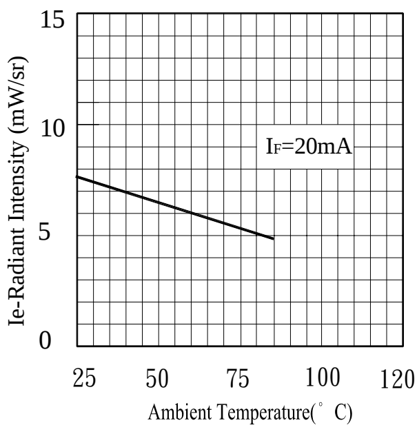
Fig.7 Radiant Intensity vs. Ambient Temperature( ^\circ C)
