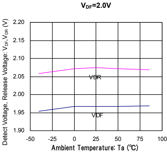
( 9 ) Detect Voltage, Release Voltage vs. Ambient Temperature
