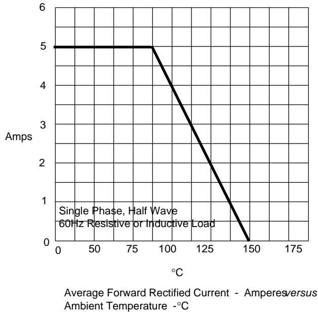
Figure 3 Forward Derating Curve
