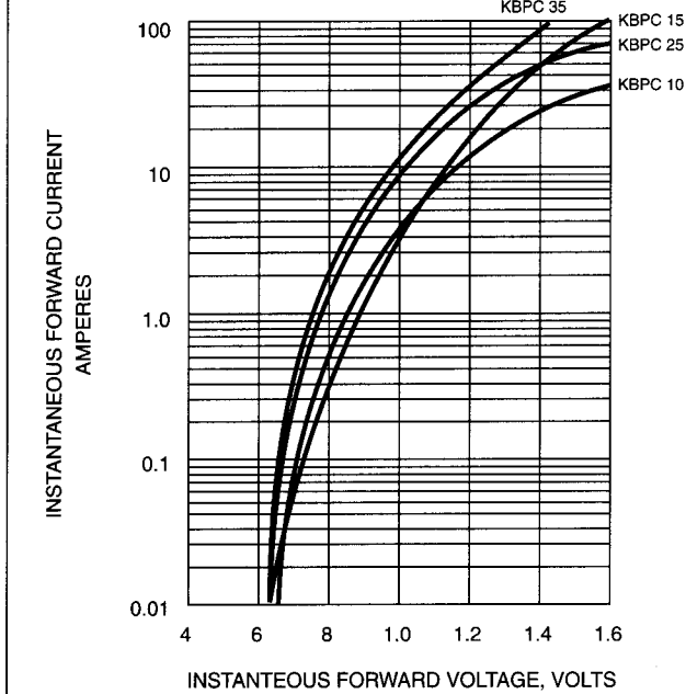
FIG. 3-TYPICAL FORWARD CHARACTERISTICS
