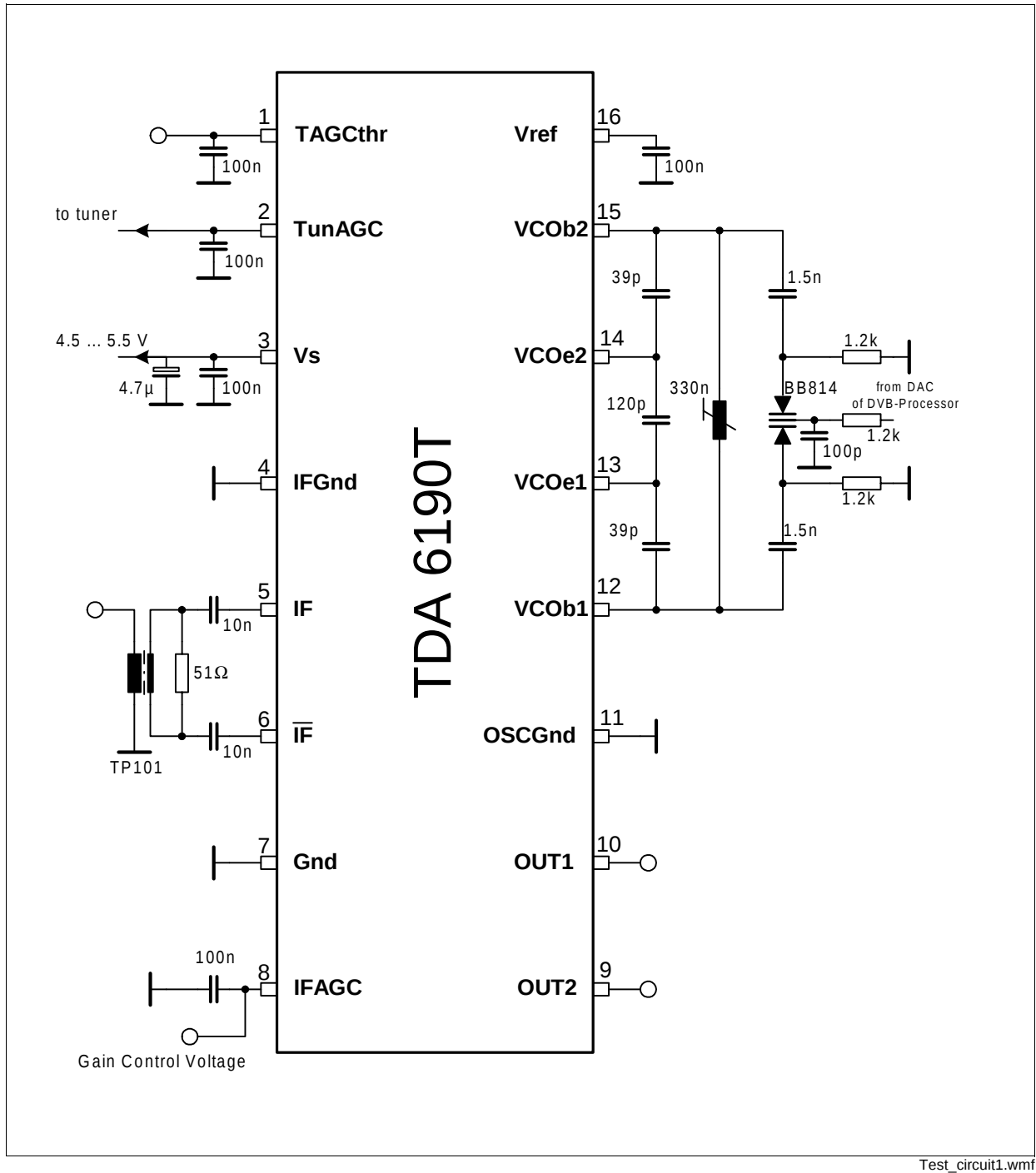
Figure 4-1 Test Circuit
