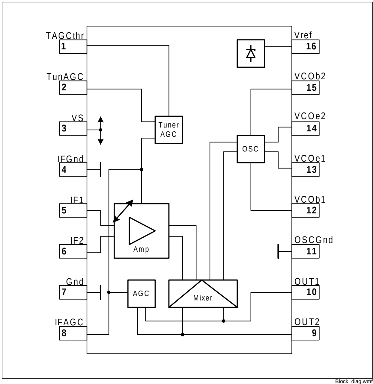
Figure 2-3 Block Diagram
