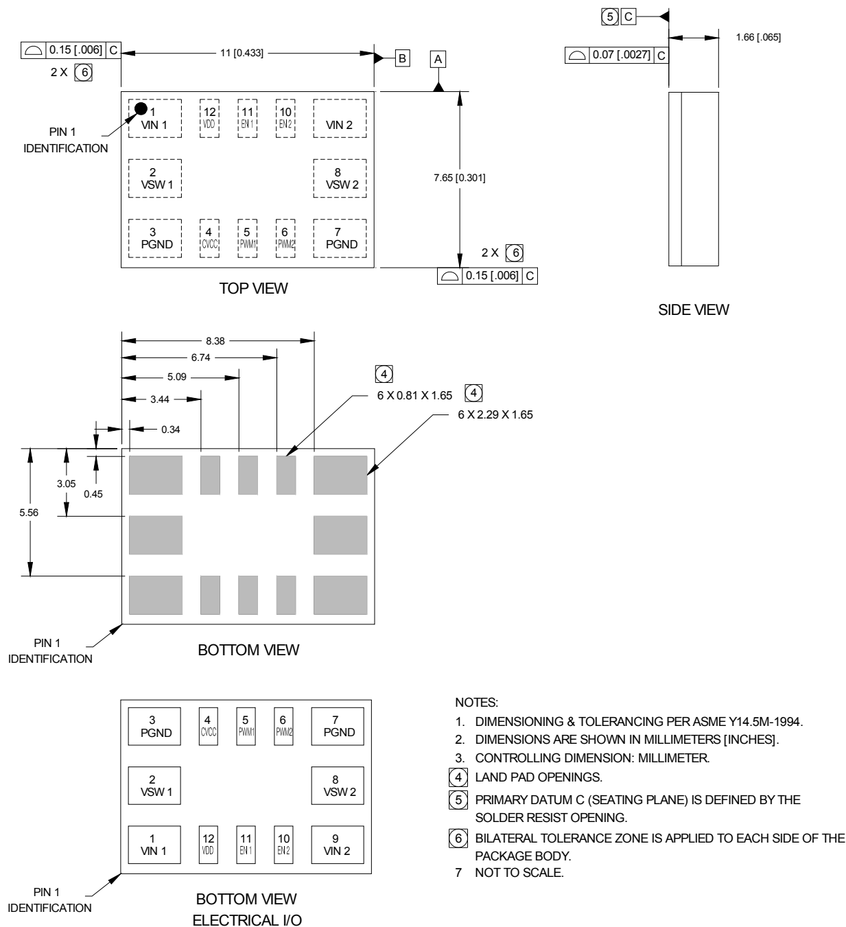
Figure 13 Mechanical Outline Drawing
