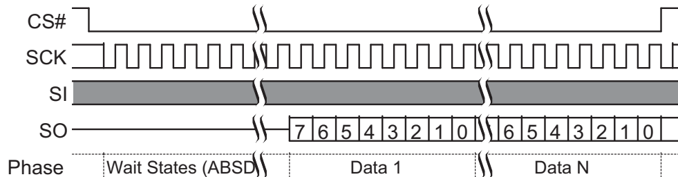
Figure 63. AutoBoot Sequence (CR1[1]=0)
