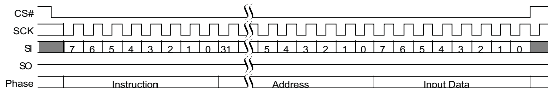
Figure 111. DYBWR (E1h) Command Sequence
