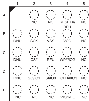
Figure 41. 24-Ball BGA, 5 x 5 Ball Footprint (FAB024), Top View
