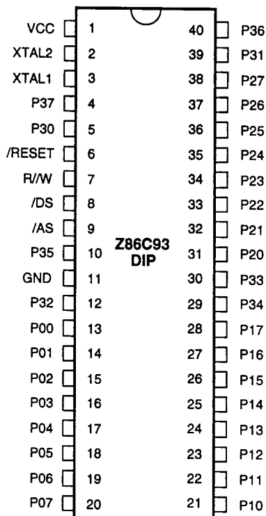
40-Pin DIP Package (20 MHz)
