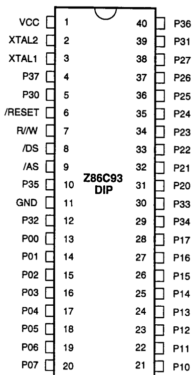
40-Pin DIP Package (25 MHz and 33 MHz)
