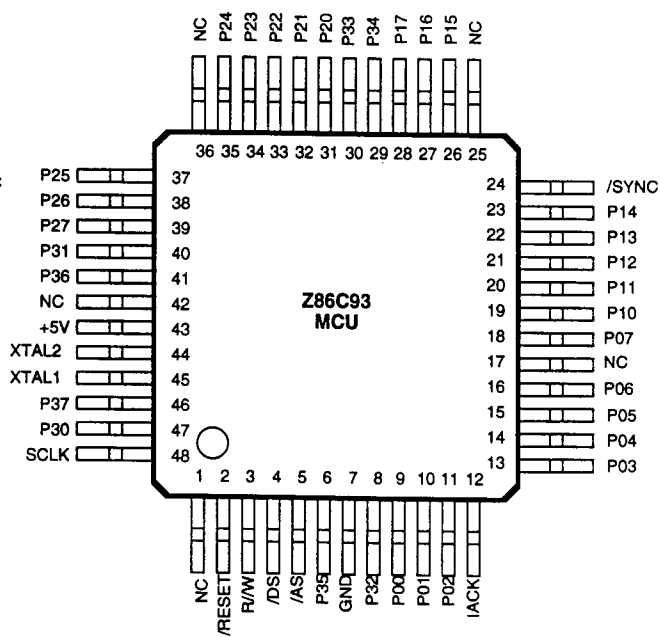
48-Pin VQFP Package (20 MHz)
