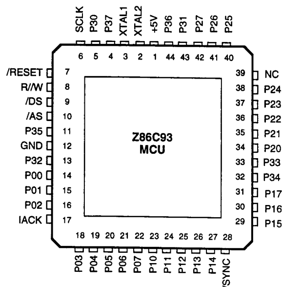
44-Pin PLCC Package (20 MHz)
