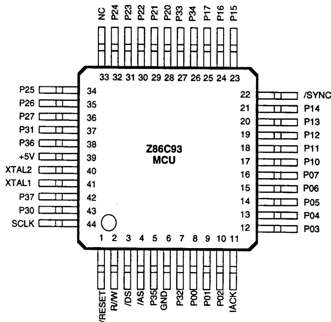
44-Pin LQFP package (20 MHz)
