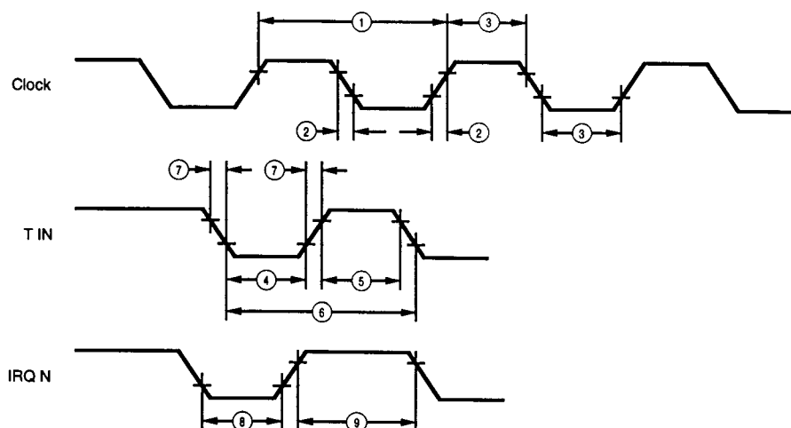
Additional Timing
