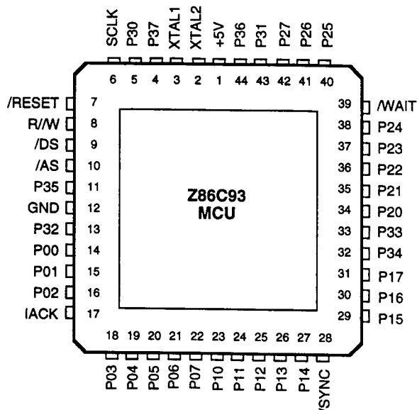
44-Pin PLCC Package (25 MHz and 33 MHz)
