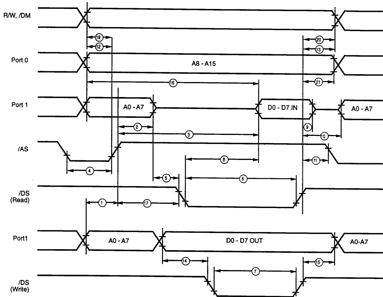
External Memory Read/Write Timing
