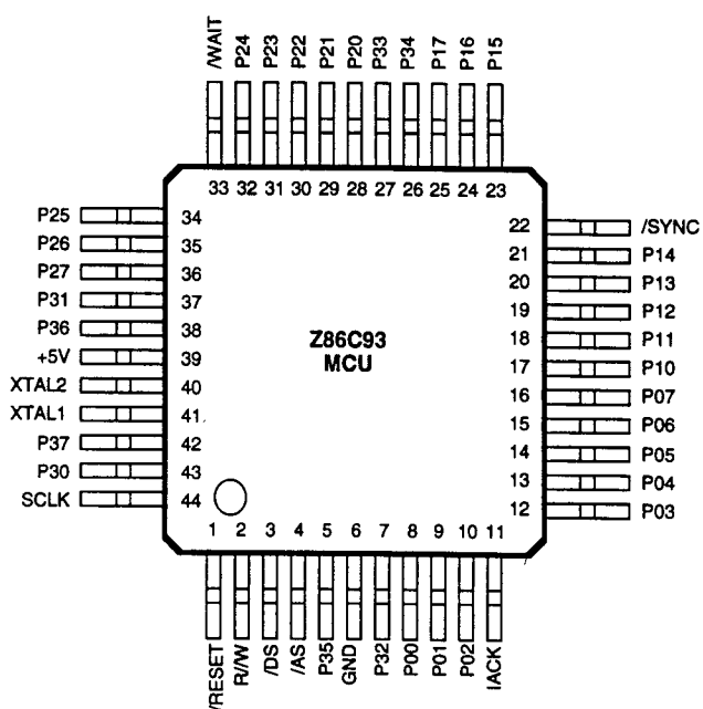
44-Pin LQFP package (25 MHz and 33 MHz)
