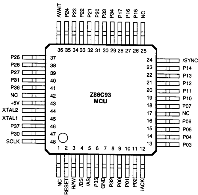
48-Pin VQFP Package (25 MHz and 33 MHz)
