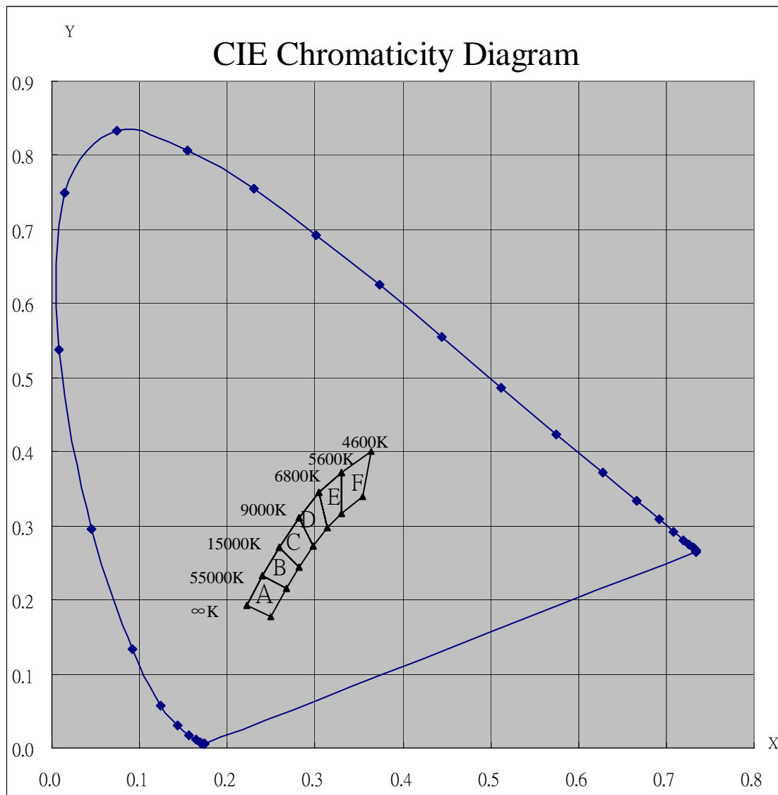
Color Ranks(IF=20mA,Ta=25℃)
