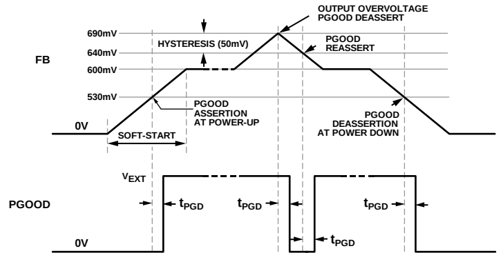
Figure 80. Power Good Timing Diagram, t_{PG} = 12 \mu s (Diagram May Look Disproportionate for Illustration Purposes.)
