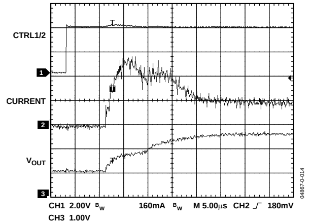
Figure 13. Soft Start Showing the Initial In-Rush Current and V_{OUT} Variation, Six LEDs @ 20 mA/LED, V_{CC} = 3.6 V
