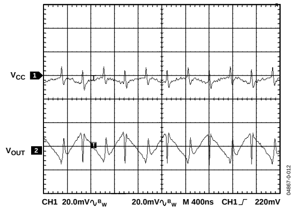
Figure 11. 1.5x Mode Operating Waveforms
