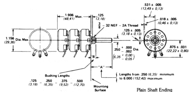
Plain or Shaft Watertight Bushing
