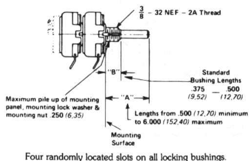
Four randomly located slots on all locking bushings.
