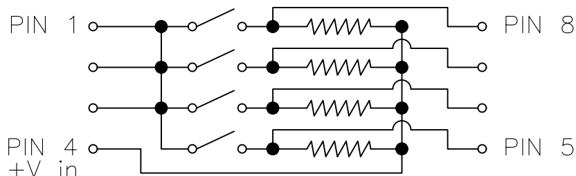
ELECTRICAL SCHEMATIC ARF SERIES ONLY
