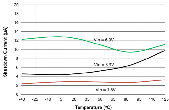
Shutdown Current
