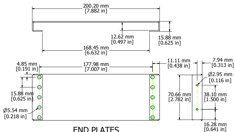
END PLATES
