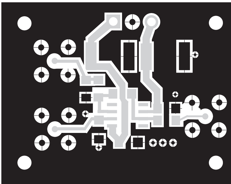
Figure 2–2. THS4051 EVM PC Board Layout – Component Side
