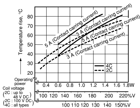
2. Temperature rise characteristics (single side stable)
