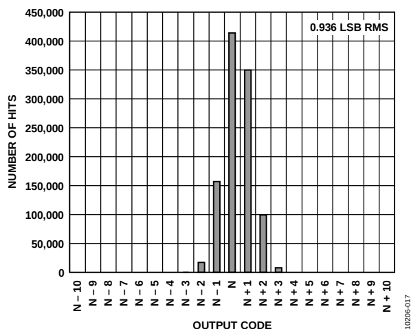
Figure 18. Input-Referred Noise Histogram, f_{\text{SAMPLE}} = 65 \text{ MSPS}
