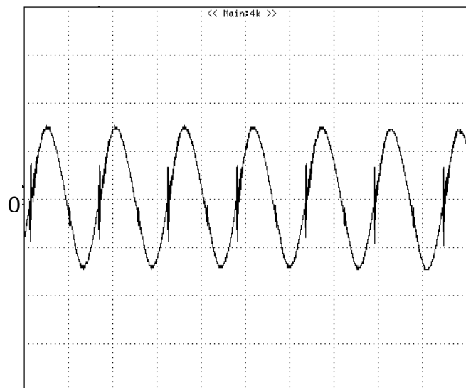
Figure 14: Output voltage ripple at nominal input voltage and rated load current ( I_o=12A ) (20 mV/div, 2 \mu s/div) Load capacitance: 1 \mu F ceramic capacitor and 10 \mu F tantalum capacitor. Bandwidth: 20 MHz. Scope measurements should be made using a BNC cable (length shorter than 20 inches). Position the load between 51 mm to 76 mm (2 inches to 3 inches) from the module.
