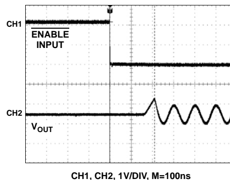
FIGURE 26. ENABLED RESPONSES
