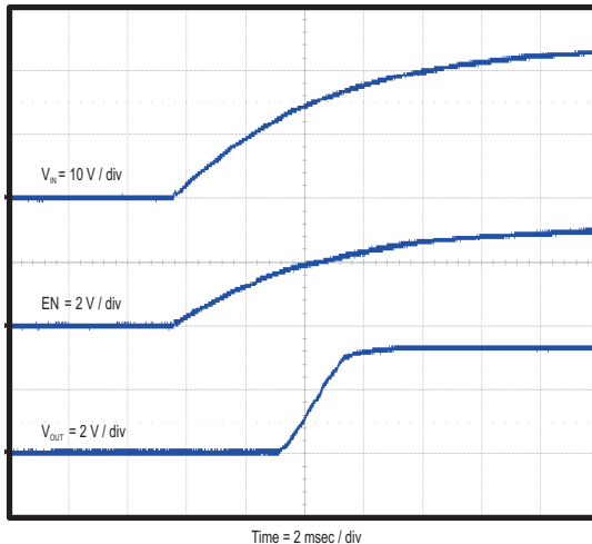
Figure 29. Start-Up With V_{IN}
