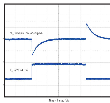
Figure 26. Load Transient
