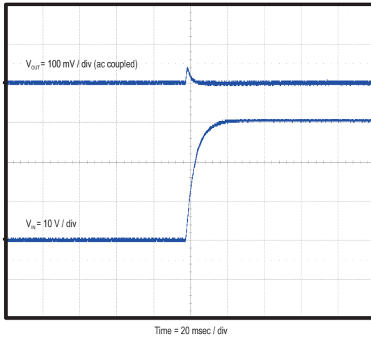
Figure 27. Line Transient
