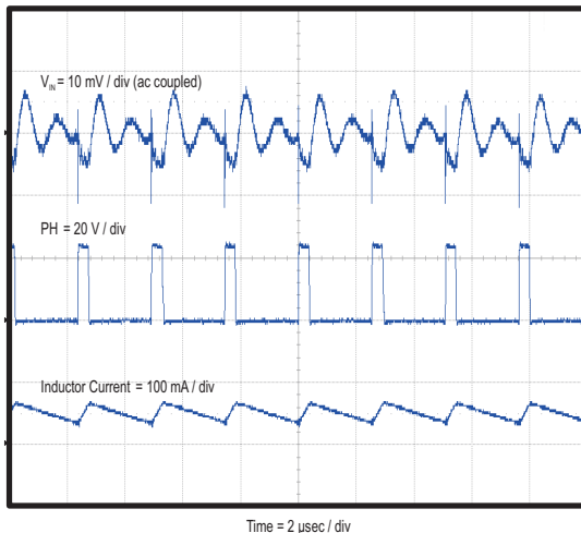
Figure 31. Input Ripple in CCM
