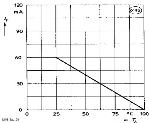
Fig. 4 Permissible Diode Forward Current vs. Ambient Temperature
