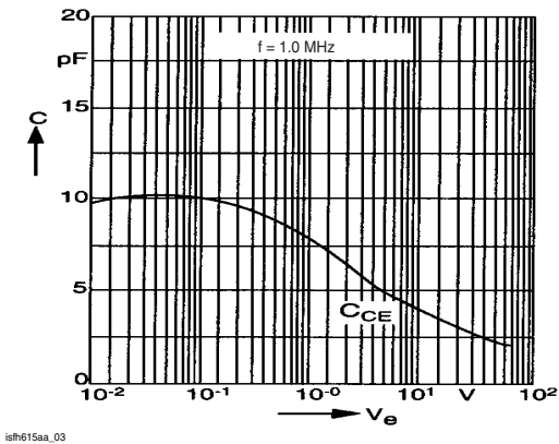
Fig. 3 Transistor Capacitance (typ.) vs. Collector-Emitter Voltage
