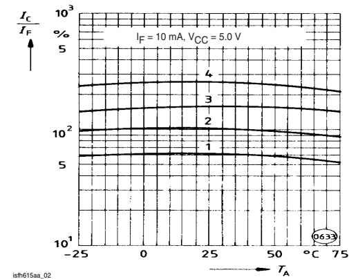
Fig. 2 Current Transfer Ratio (typical) vs. Temperature
