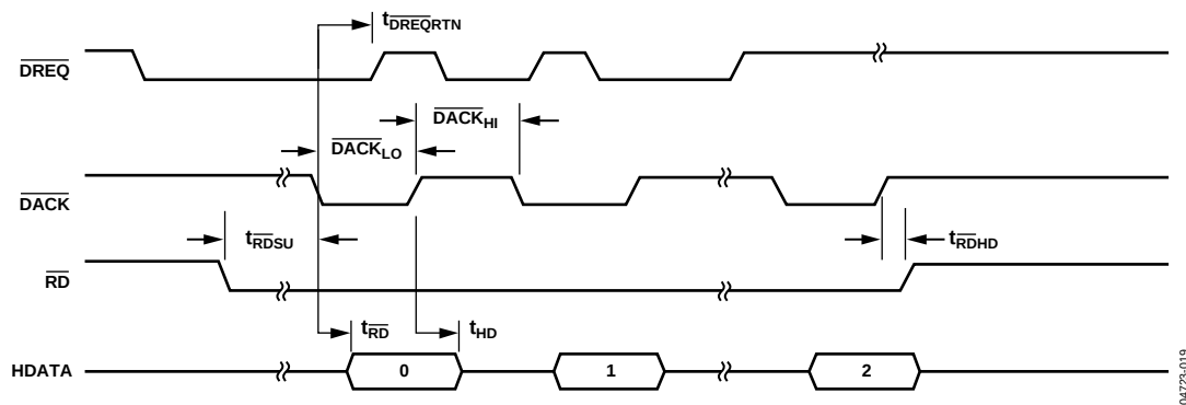
Figure 10. Single Read for DREQ/DACK DMA Mode for Assigned DMA Channel (EDMOD0/EDMOD1 <14:11> Programmed to a Value of 0000)
