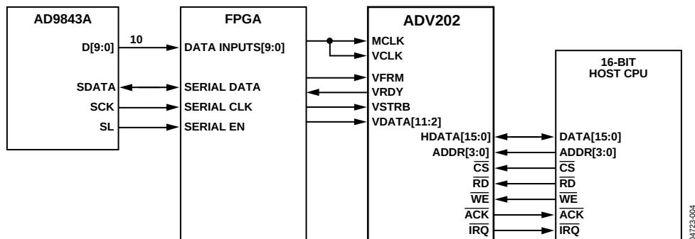
Figure 27. Digital Still Camera/Camcorder Application
