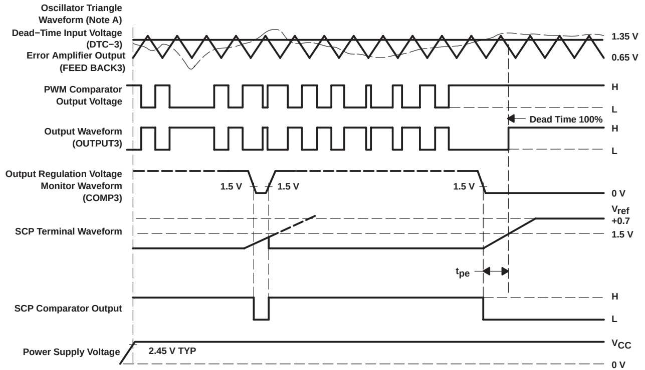
Figure 3. Timing Diagram (channel 3)
