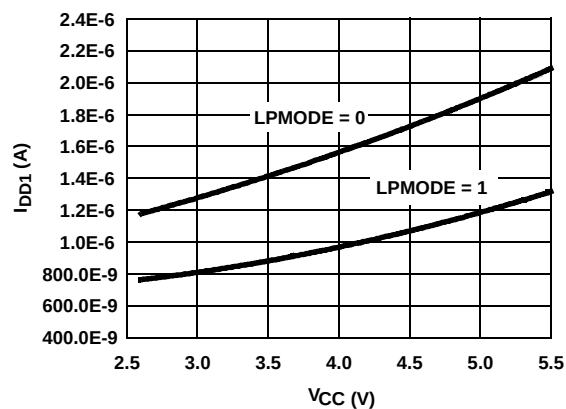
FIGURE 4. I_{DD1} vs V_{CC} WITH LPMODE ON AND OFF
